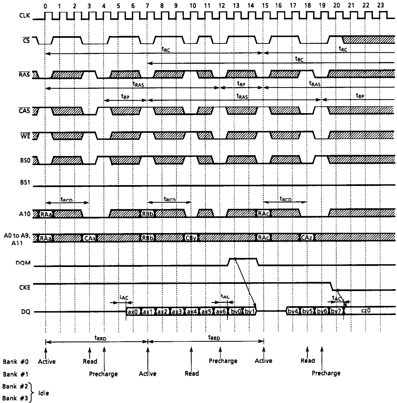
Figure 3. Interleaved Bank Read (Burst Length=8, \overline{\text{CAS}} Latency=3)
